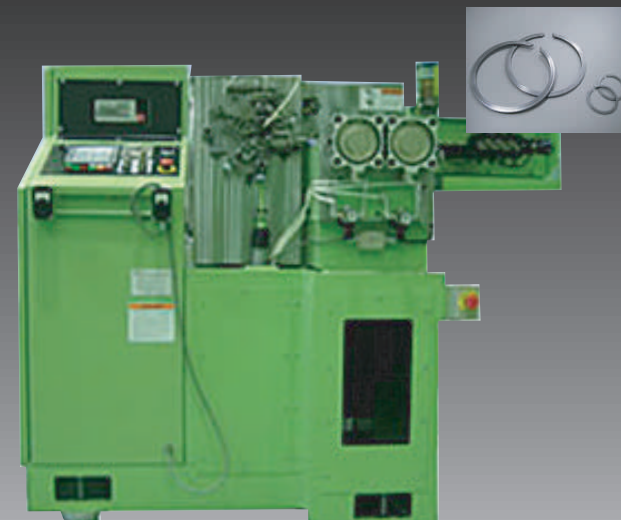
NFR-250-3 for small size of ring (φ20~60mm/Max.200spm)
